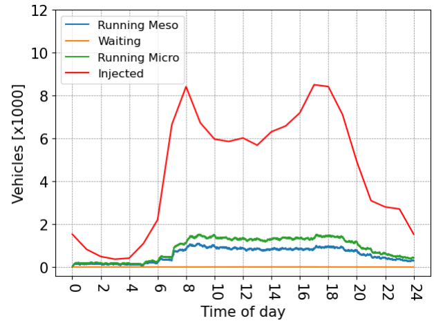
Fig. 10. Comparison between mesoscopic and non mesoscopic simulations.
