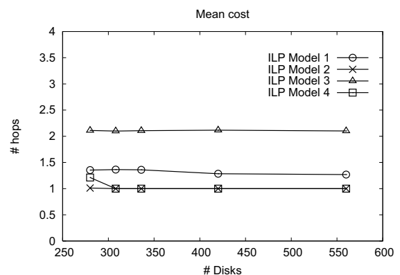
Fig. 4. Mean cost, i.e. the maximum path length in number of hops, for ILP models
