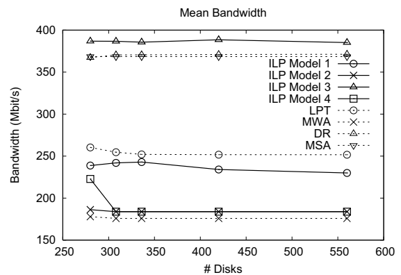
Fig. 3. Mean link bandwidth
