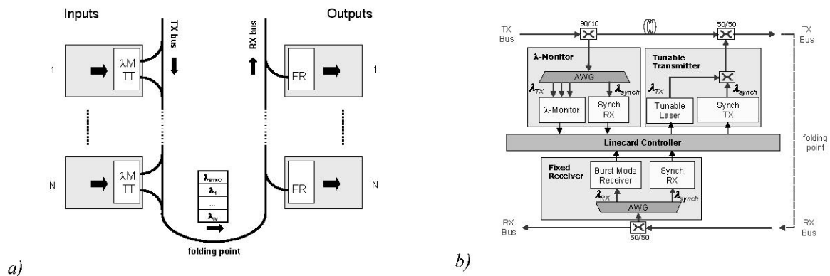
Figure 1. a) Interconnection architecture b) Line card architecture.
