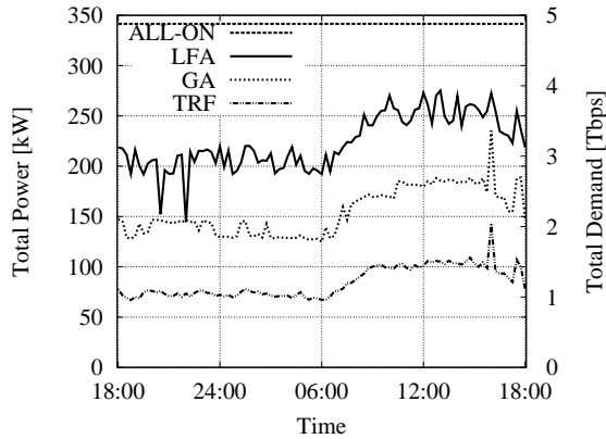
(a) Power consumption follows the traffic pattern for LFA and GA.
